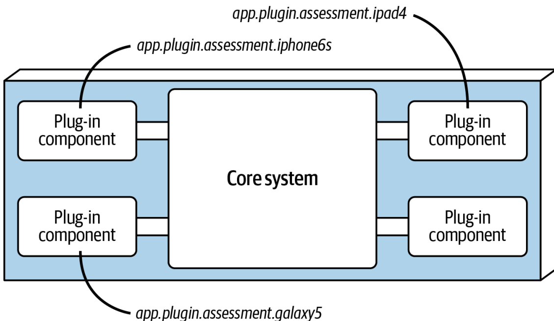
Figure 13-5. Package or namespace plug-in implementation
