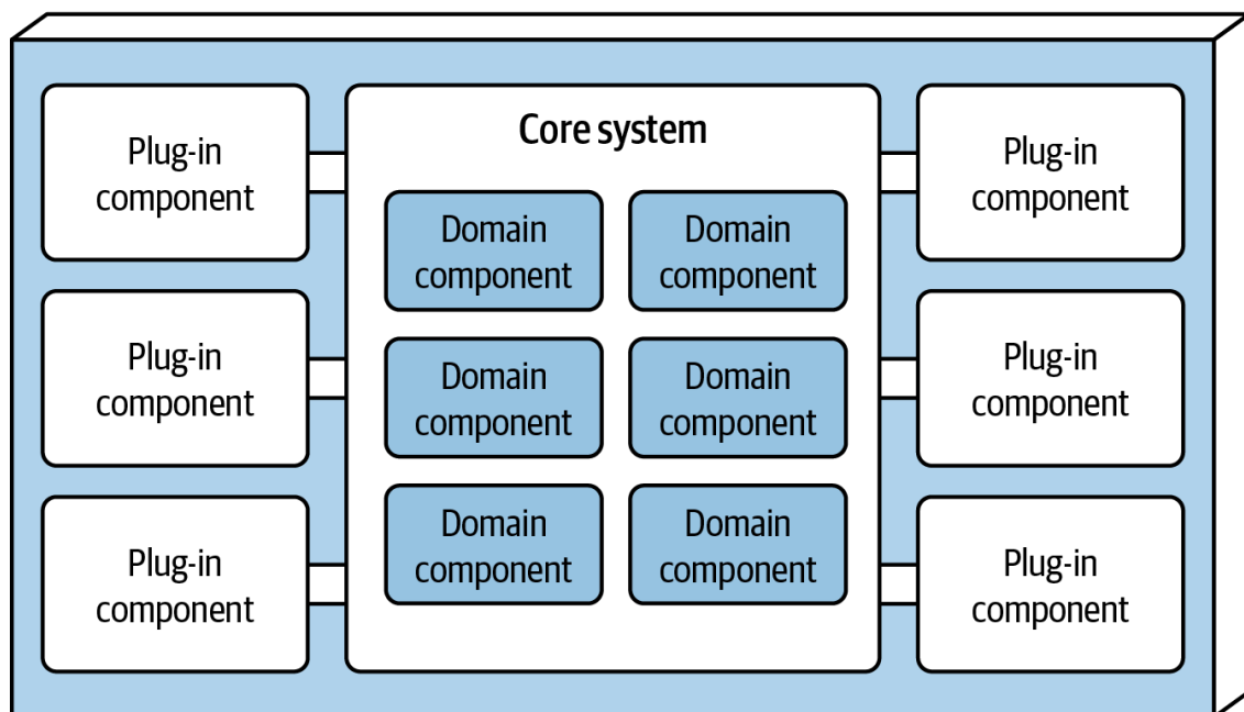
Modular core system (domain partitioned)
