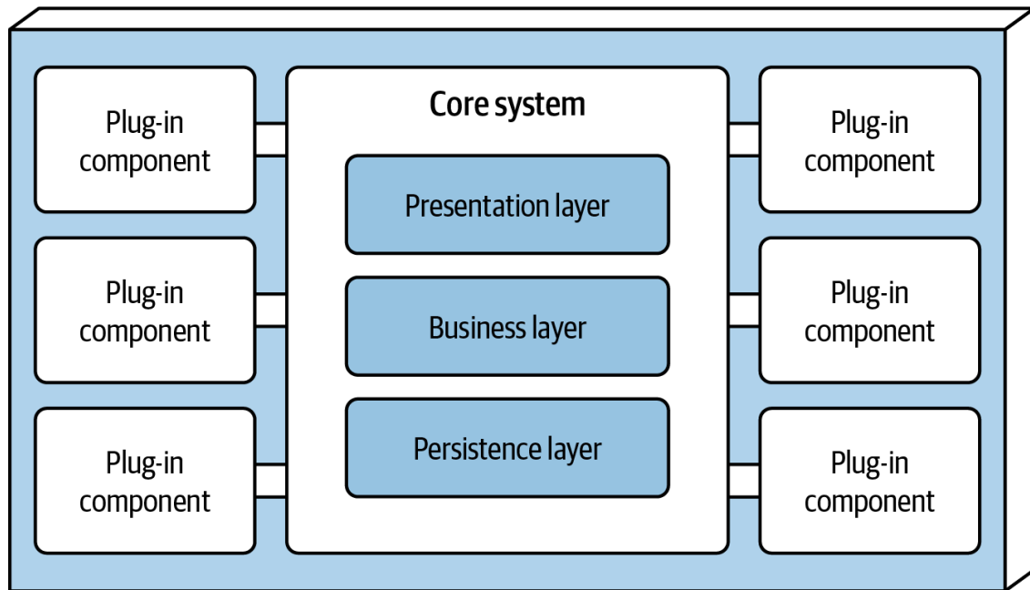
Layered core system (technically partitioned)
