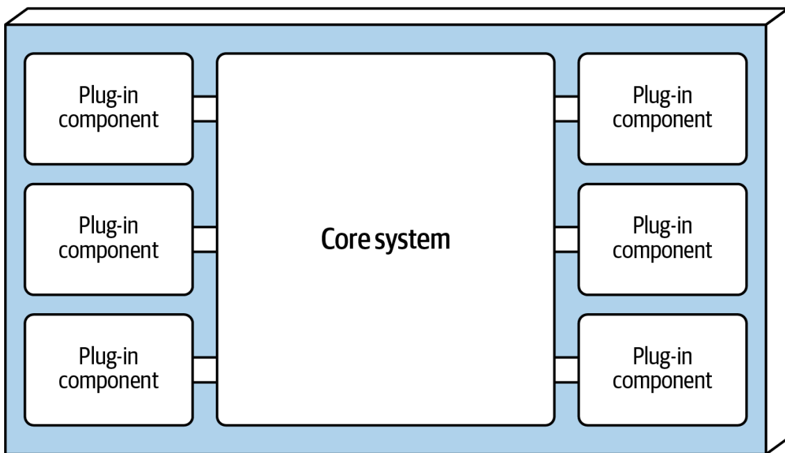
Figure 13-1. Basic components of the microkernel architecture style
