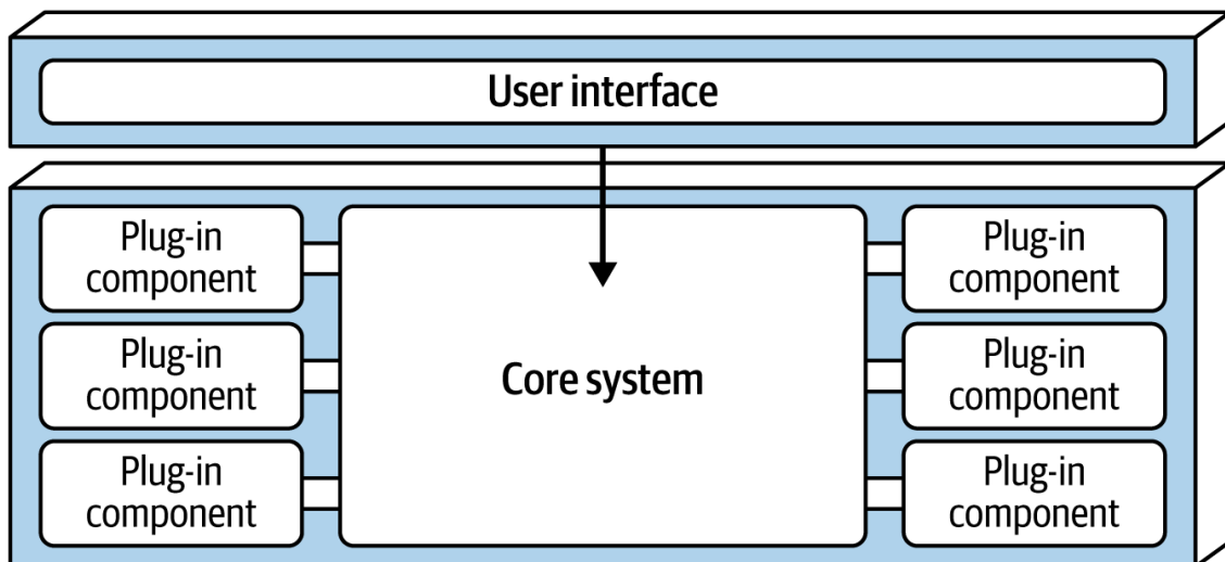
Separate user interface (multiple deployment units)
