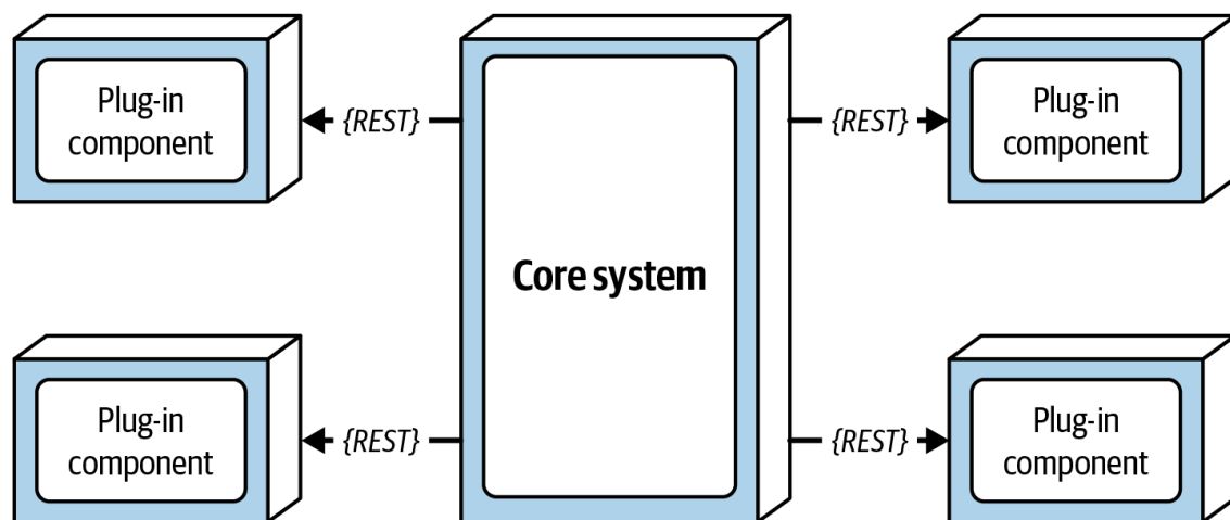
Figure 13-6. Remote plug-in access using REST
