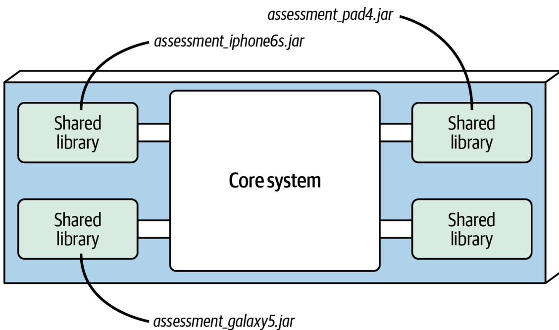
Figure 13-4. Shared library plug-in implementation
